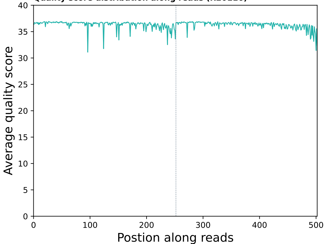
Quality score distribution along reads (R20116)
